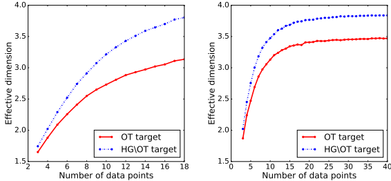
Figure 3: Average effective dimension of the learner’s weights over OT and HG-non-OT target grammars as a function of n , for rounding harmony (left) and syllable types (right) data.
