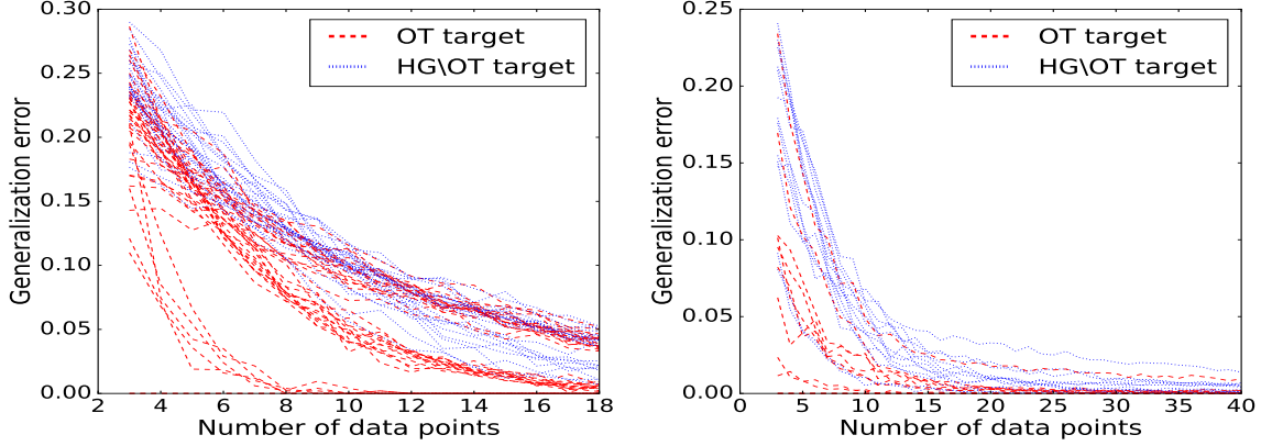
Figure 4: Generalization error Err(n, G) as a function of n , for rounding harmony (left) and syllable types (right) data, for each OT target grammar G (red line) and each HG-non-OT target grammar G (blue line).
