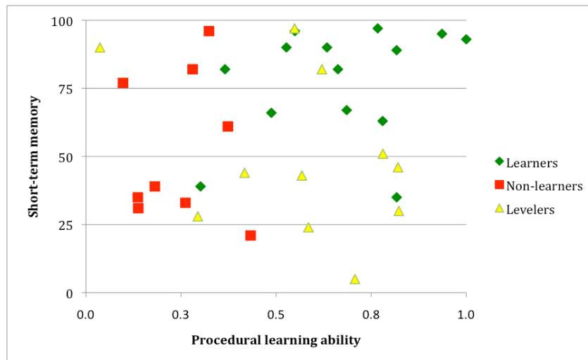
Figure 7: Scatter plot showing participants' performances on both procedural learning and short-term memory tasks, grouped by language-learning ability.
