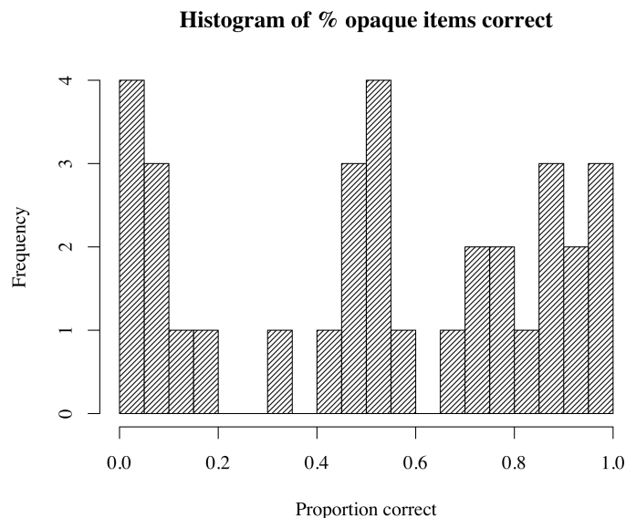
Figure 3: Histogram of percent of opaque items answered correctly
