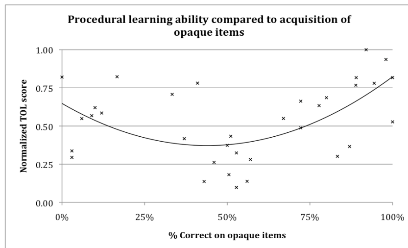
Figure 6: Performance on test of procedural memory versus performance on opaque items.
