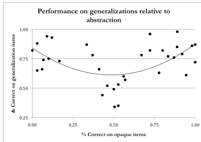
Figure 4: Performance on acquiring generalizations relative to the opaque interaction
