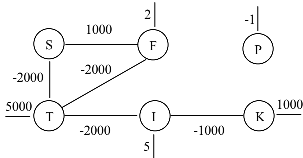
Figure 4: First order network with one hidden unit T
