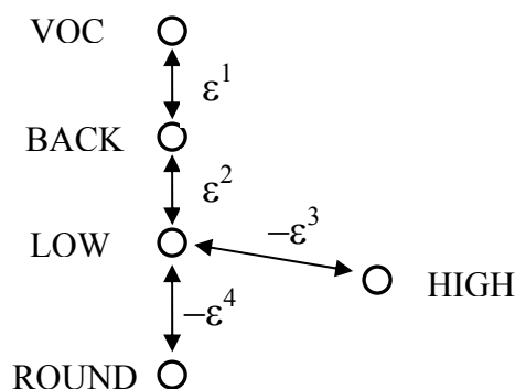
Figure 6: Hopfield network with exponential weights representing the generic knowledge 21 of a phonological agent
