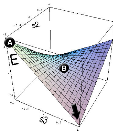
Figure 5: Energy landscape for calculating the asymptotic updates of \langle 1 \ 0 \ 0 \rangle . Starting points for energy minimization: A for the Boolean option, B for the DeMorgan option.
