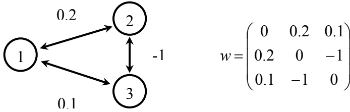
Figure 1: Symmetric network with weight matrix
