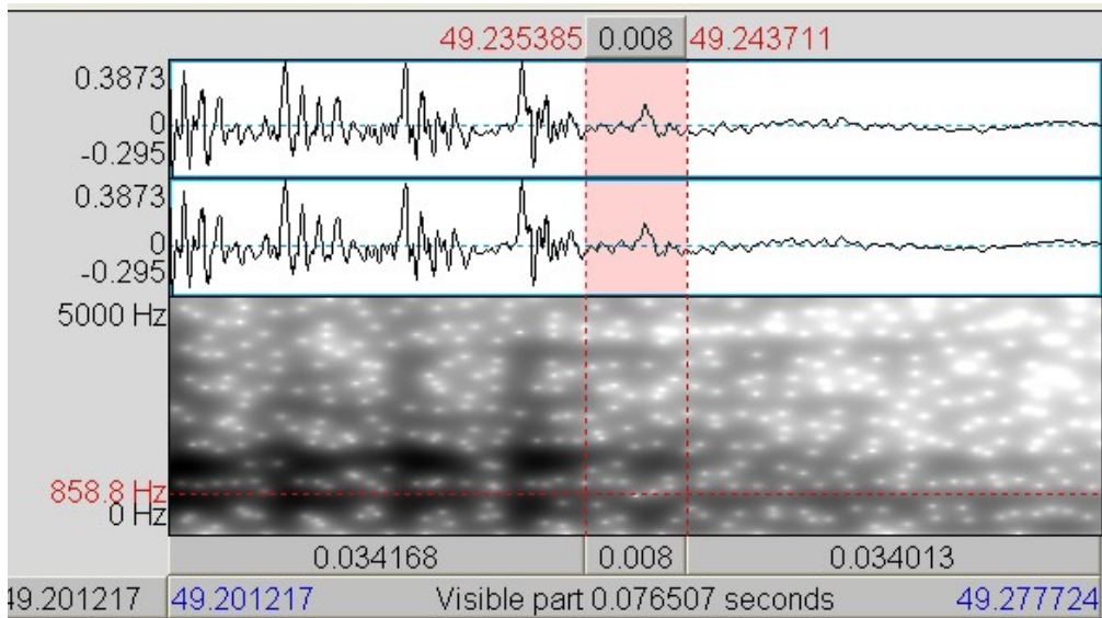
Figure 2.9. Hindi ata [a:ta] ‘he comes’. VC transition shown; stop prevoicing highlighted (8 ms).
