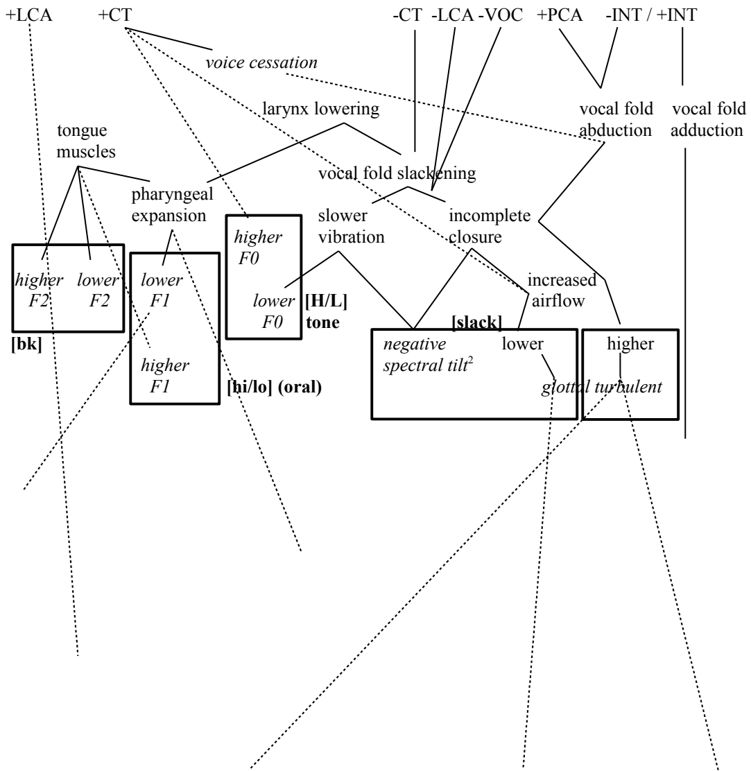
Figure 3.2. Suggested maximum number of features (bold) that can be simultaneously assigned in the phonetic space shown, with some exclusions at bottom (see discussion). Boxes show feature-cue assignment.
